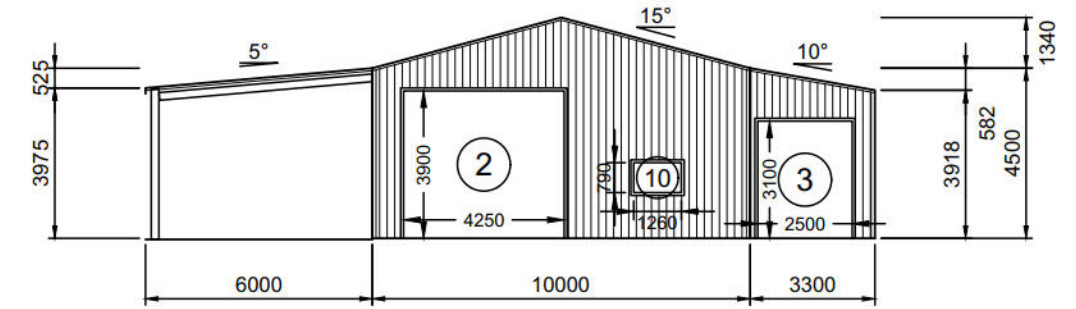
3 REAR BUILDING ELEVATION SCALE: 1:200
