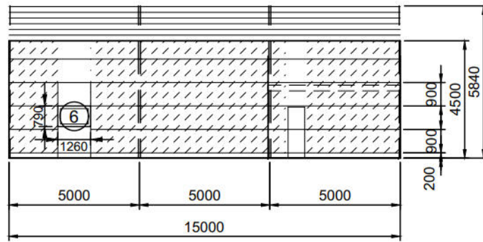
2 SIDEWALL B FRAMING ELEVATION SCALE: 1:200
