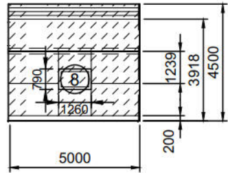
2 LEANTO B FRAMING ELEVATION SCALE: 1:200
