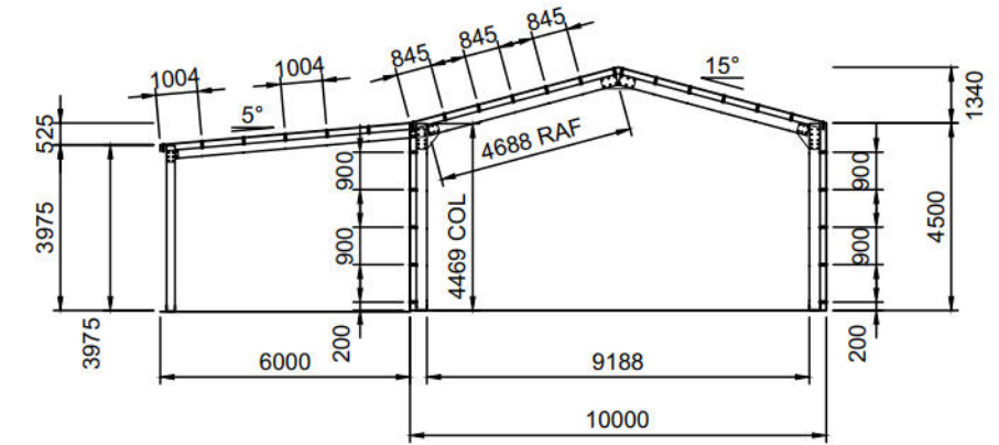
6 INTERNAL FRAMING ELEVATION SCALE: 1:200
