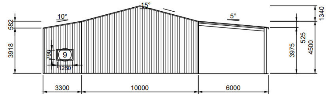
4 FRONT BUILDING ELEVATION SCALE: 1:200
