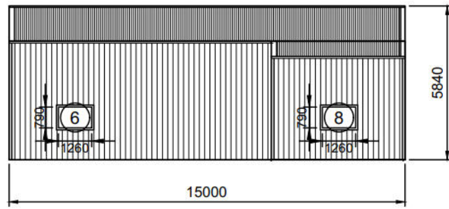
2 SIDEWALL B BUILDING ELEVATION SCALE: 1:200
