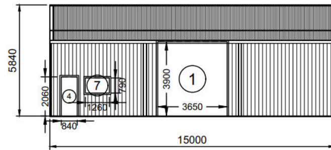
1 SIDEWALL A BUILDING ELEVATION SCALE: 1:200
