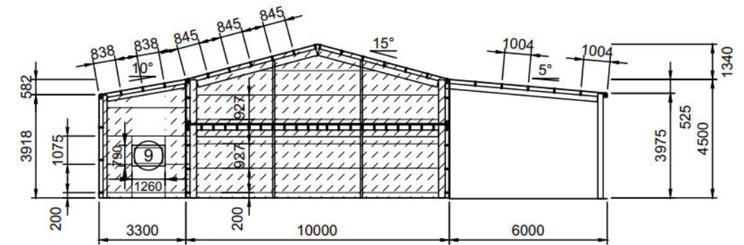
4 FRONT FRAMING ELEVATION SCALE: 1:200
