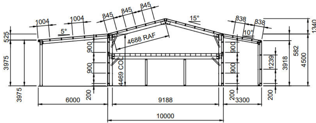
5 INTERNAL FRAMING ELEVATION SCALE: 1:200
