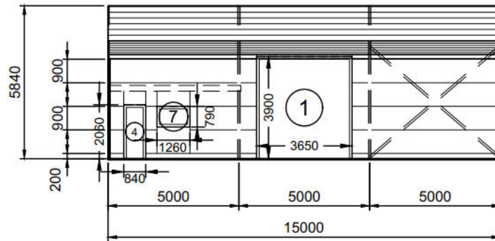
1 SIDEWALL A FRAMING ELEVATION SCALE: 1:200
